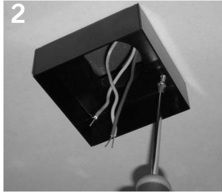
2 Install junction box cover as shown.
