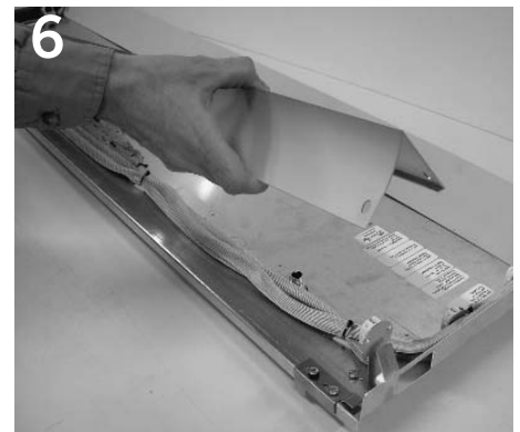
6 Slide reflector to one side and lift. Remove both reflectors.
