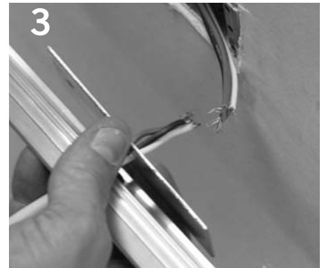
3 Make electrical connection. NOTE: Fixture backplate should be between channel back and junction box.
