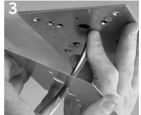
3 Position coverplate on mounting plate.
