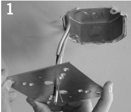
1 Slide mounting plate over pre-installed octagonal junction box.
