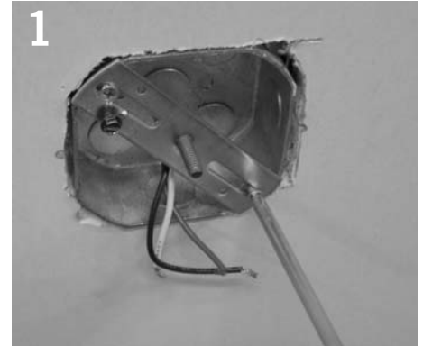
1 Install j-box strap and 1/4-20 stud to j-box.
