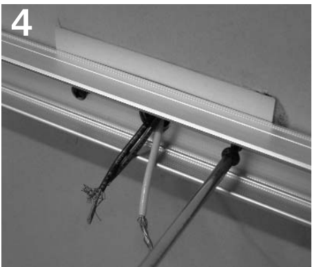
4 Level and secure trim plate and back channel to junction box.
