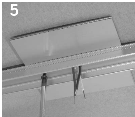
5 Secure trim plate and back channel to junction box plate.
