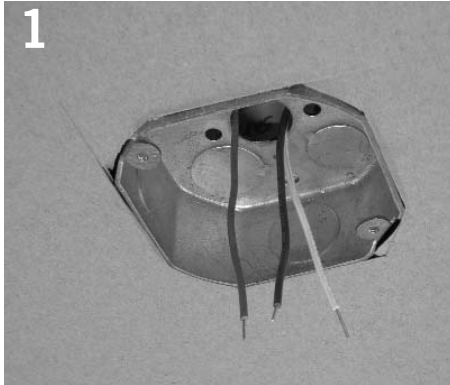
1 Install octagonal junction box into ceiling.
