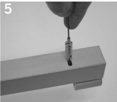
5 Insert cables into grippers on top of luminaire.
