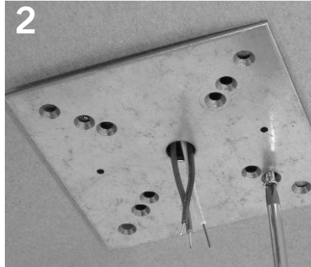
2 Secure junction box cover plate to junction box. Route building supply wires through center hole in plate.
