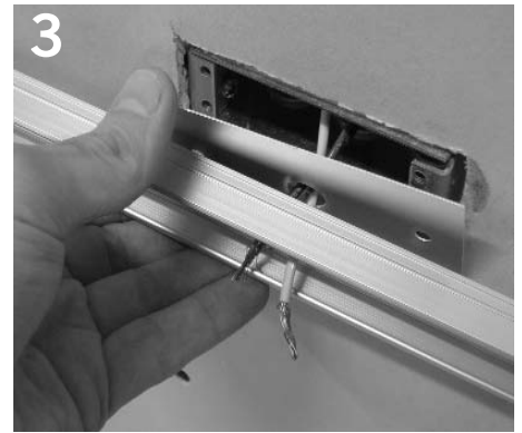
3 Insert building supply wires through center hole in trim plate and through center hole in back channel. Trim plate should be between back channel and junction box, as shown.
