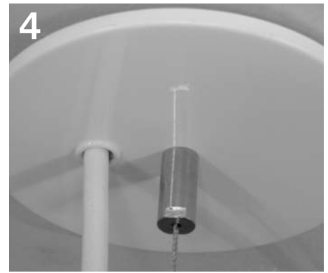
4 Secure canopy by tightening barrel nut onto stud. Repeat the same steps (without electrical cord) for the support end of luminaire..
