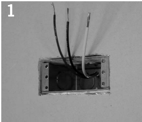
1 Install Energie junction box into wall in orientation of desired luminaire direction.
