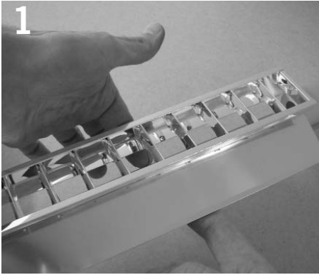
1 Compress spring clip near each end of baffle. Lift baffle away from luminaire body.
