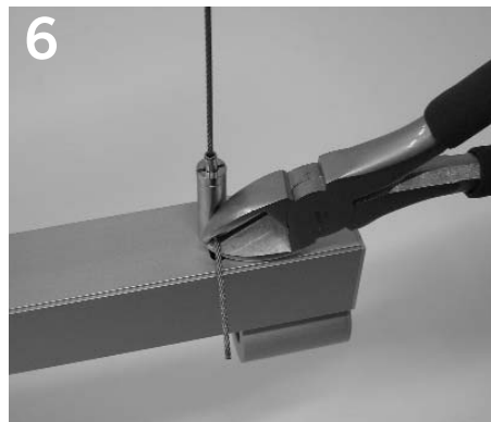
6 Adjust luminaire to desired height and trim excess cable.
