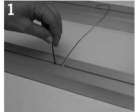
Adjust cable stops (4) to desired position along fixture extrusion.
