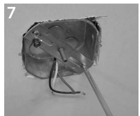
Install j-box strap and 1/4-20 stud to j-box.
