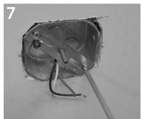
Install j-box strap and 1/4-20 stud to j-box.
