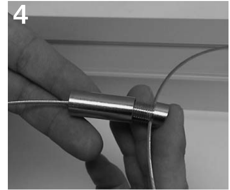
Lace swaged cable through female end of suspension mechanism and screw to male end.
