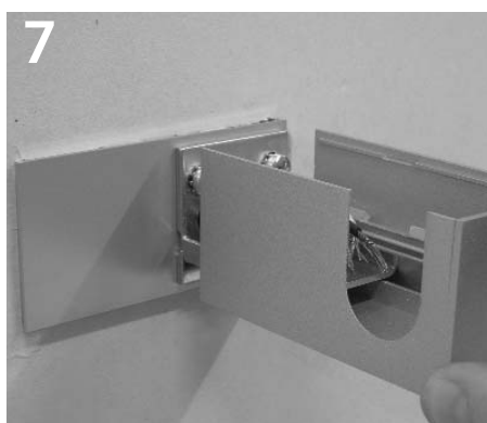
7 Slide end block onto support bracket. NOTE: Opening in end block should face in direction of blank portion of trim plate, as shown.
