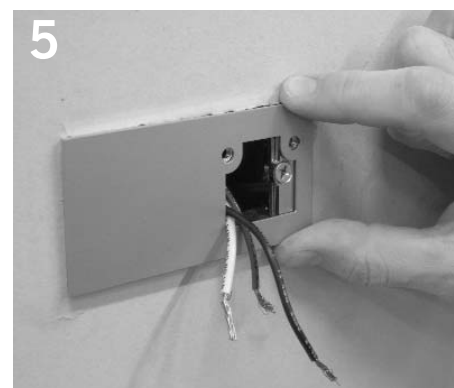
5 Place trim plate over mounting plate and route connector cord through opening.
