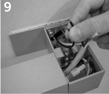
Install luminaire body per instructions. Make EMC electrical connection.
