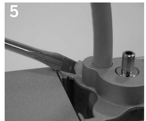
5 Tighten strain relief screw to secure feed cord.
