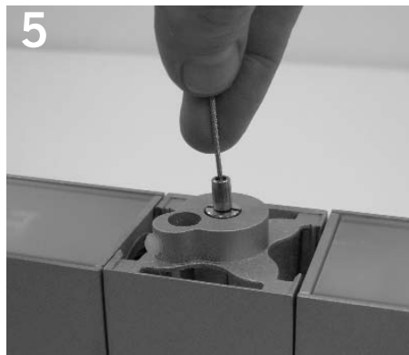
5 Install suspension cable into gripper in connector/ corner/ end block. NOTE: Gripper securing ring may need to be loosened prior to inserting cable.
