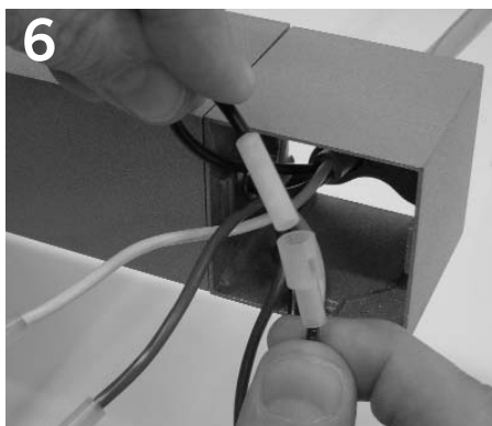
6 Connect like-colored electrical leads. Push connections back into luminaire body.
