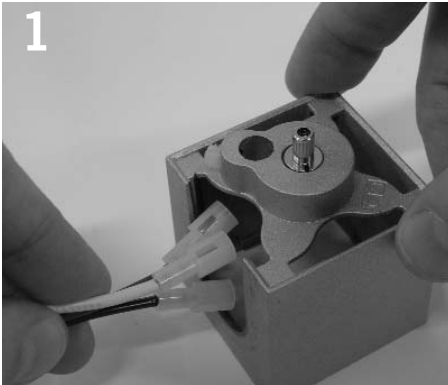
1 Route connection leads into end block.
