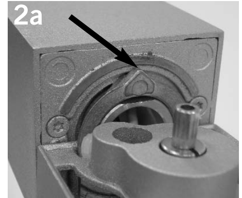
2a NOTE: To attach endblock, arrow on rotation bushing must be oriented away from end block, as shown.
