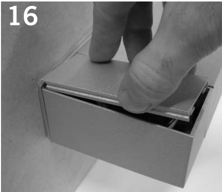
16 Snap end block covers into place. NOTE: Cover lip should face wall.
