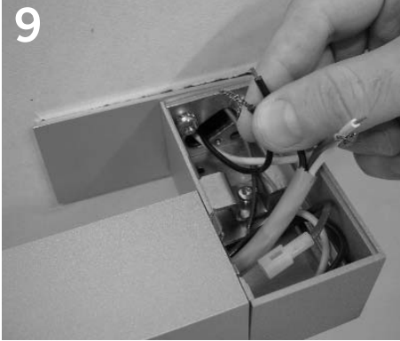
9 Install luminaire body per instructions. Make EMC electrical connection.
