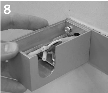
8 Slide end block onto support bracket. NOTE: Opening in end block should face in direction of blank portion of trim plate, as shown.
