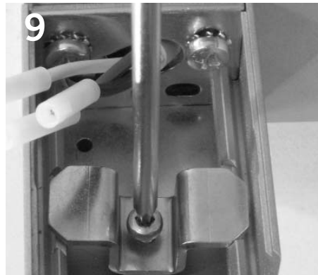
9 Rotate support bracket lock to engage end block, as shown. Tighten screw to secure.
