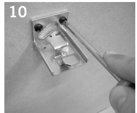
10 Install support bracket at opposite end of luminaire run with (2) #10 screws (not provided). Level bracket and tighten screws. NOTE: Mid-run joiner installed in same manner.
