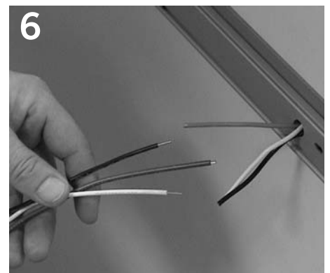
6 Make electrical connection and push connection through coverplate and mounting plate into junction box.
