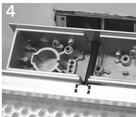
4 Install fixture over mounting screws by sliding head of screws into key holes in fixture back box.
