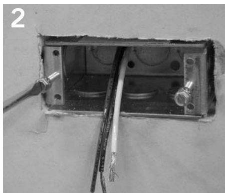
2 Install mounting screws with washers in center hole on each side of Energie junction box. Do not tighten screws.
