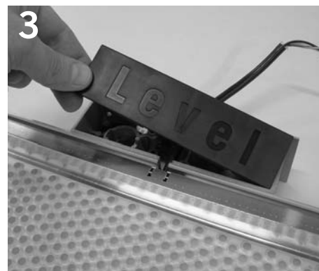
3 Remove plastic cover plate from fixture back box.
