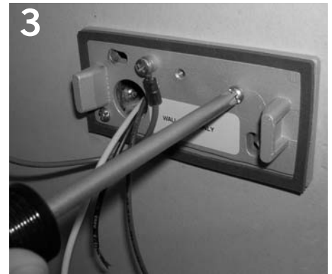
3 Attach backplate to j-box with two screws and seal to wall with clear silicone caulk.
