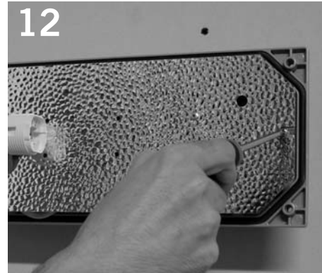
Replace reflector. Secure by tightening (2) retaining screws.
