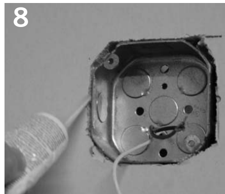
8 If fixture is to be mounted in a wet location, add silicone or similar sealant around edge of junction box.
