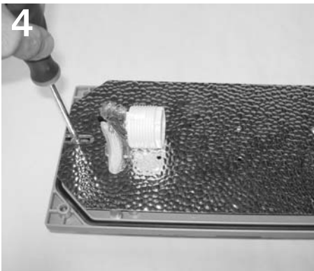
4 Loosen (2) reflector retaining screws.
