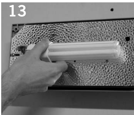
Install lamp as specified on relamp label.
