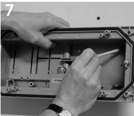
7 Use lower housing to mark mounting hole locations. Mount lower housing to wall. (Note: Reflector removed for clarity; will remain attached)
