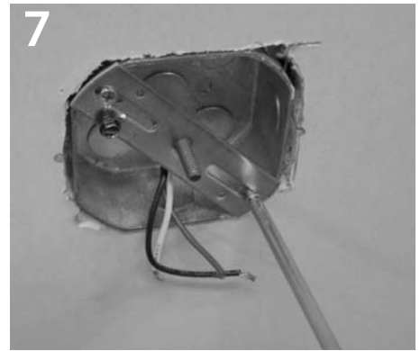
7 Install j-box strap and 1/4-20 stud to j-box.
