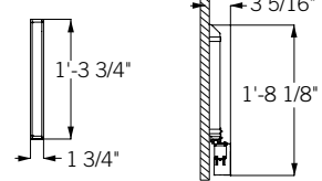
ZENN LED
