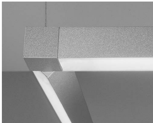
Rotation at the corners is limited. One lighting element must be in the 0°, 90°, 180° or 270° position to enable the other lighting element to rotate through the entire 360° range.
